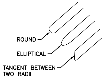
OPTIONAL DESIGN FOR GRATE OPENING ENDS
